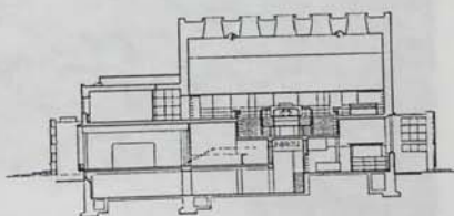
13 Library, Viipuri, 1934. Side view of main entrance, lecture hall block.
